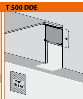
T 500 DDE Springless vertical rail system
