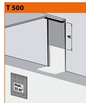
T 500 Vertical rail system
