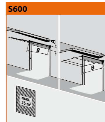
S600 Helix S600 Horizontal track system
